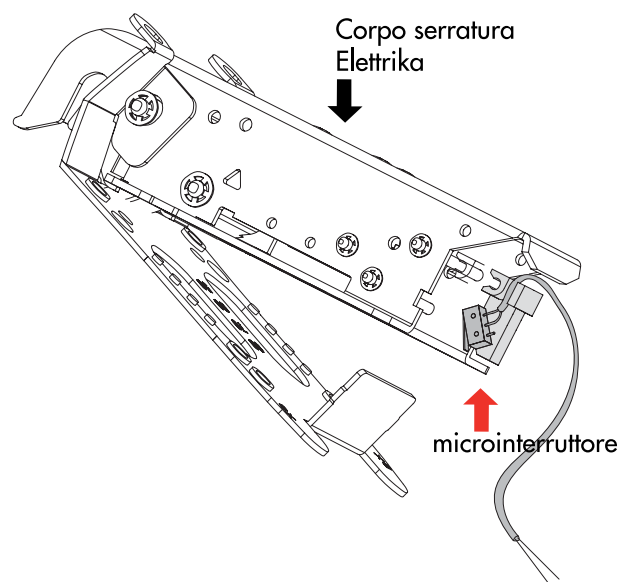
Microswitch installation diagram
